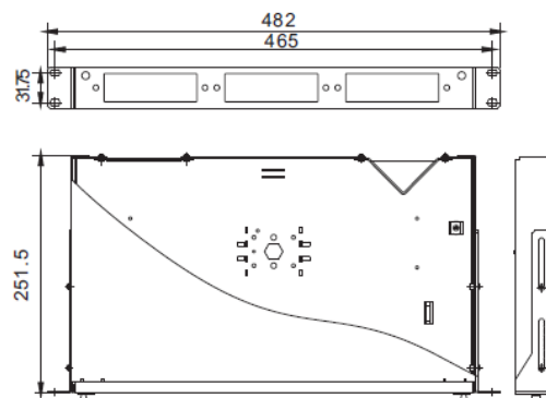
Fiber Patch Panel, 18 ports
