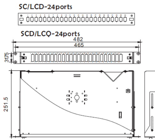
Fiber Patch Panel, 24/48 ports
